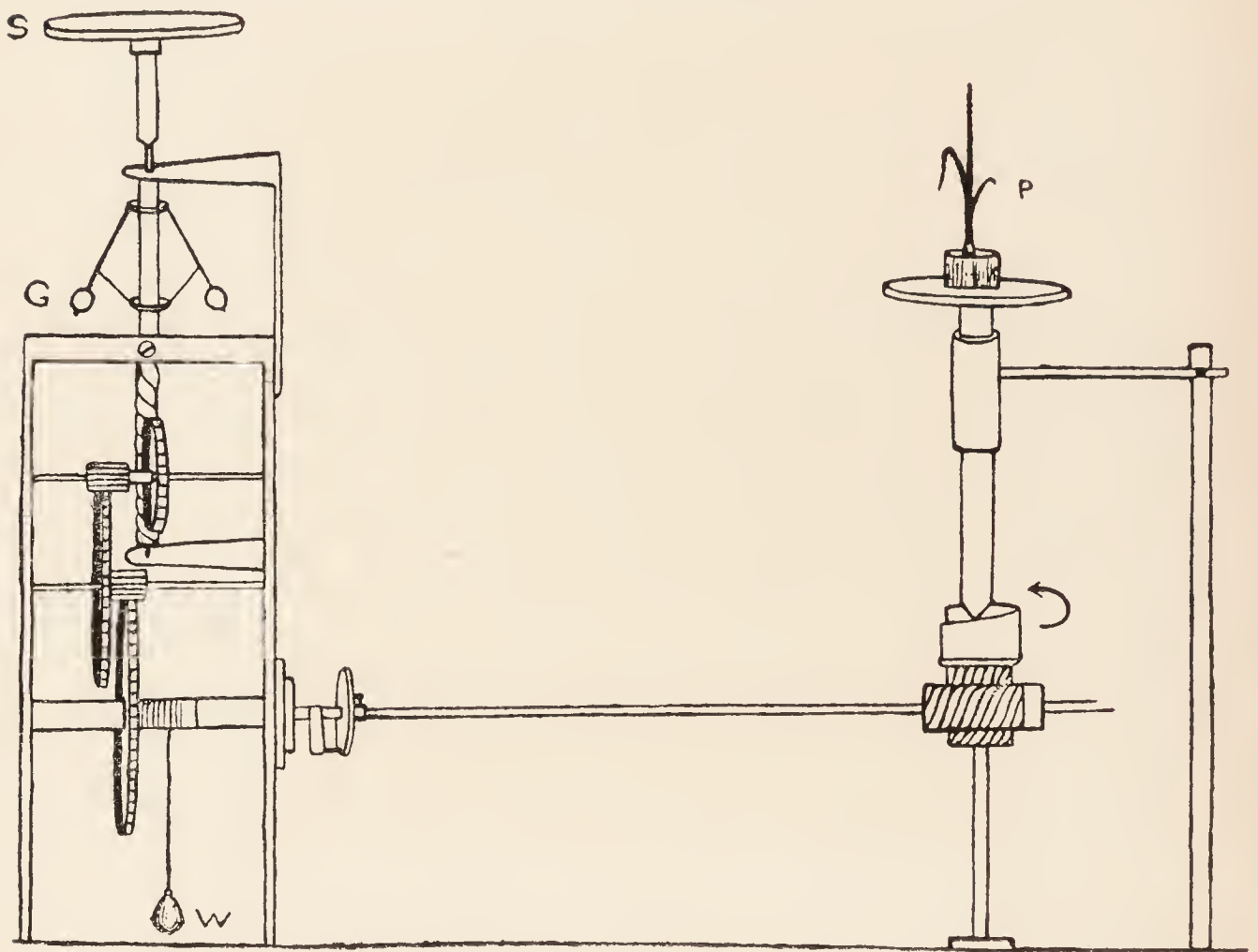
FIG. 19.—The Balanced Crescograph. Compensation of growth-movement produced by equal subsidence of the holder containing the plant (P). Adjusting screw (S) regulates the speed of the governor (G). W, heavy weight actuating clock-work.
